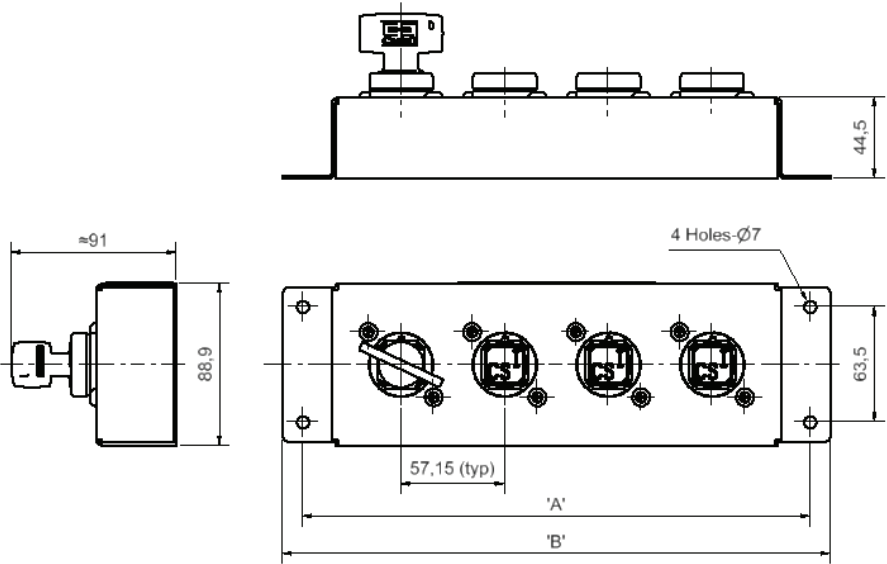
4 Front Exchange Box Shown - 1 Key In, 3 Keys Out
