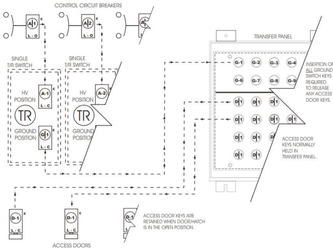
Precipitator scheme with single output transformer rectifiers.
